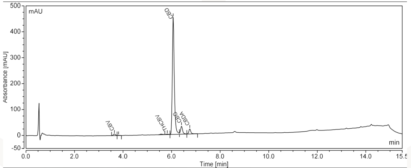
CROMATOGRAMA [MC092022-009]
