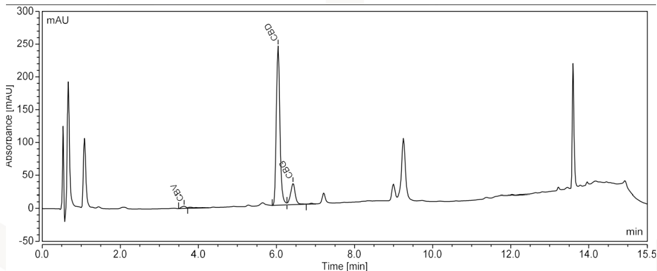
CROMATOGRAMA [MC092022-005]
