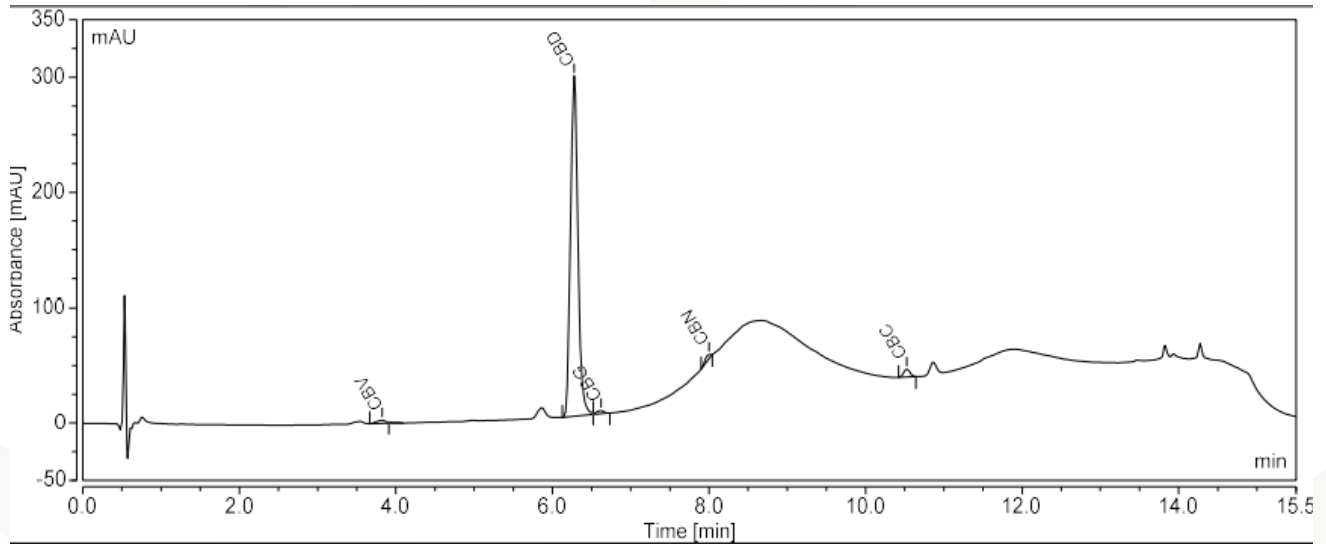
CROMATOGRAMA [MC082022-038]
