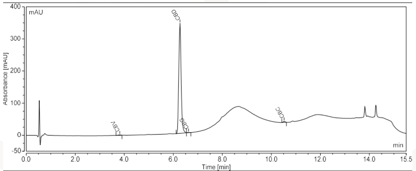
CROMATOGRAMA [MC082022-035]
