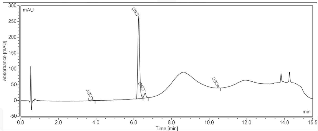
CROMATOGRAMA [MC082022-034]
