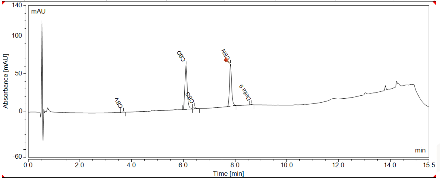
CROMATOGRAMA [MC012023-023]
